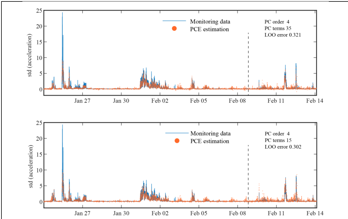
Figure 4.5. (Top) PCE model estimates for three input variables; (Bottom) PCE model estimates for two input variables;
