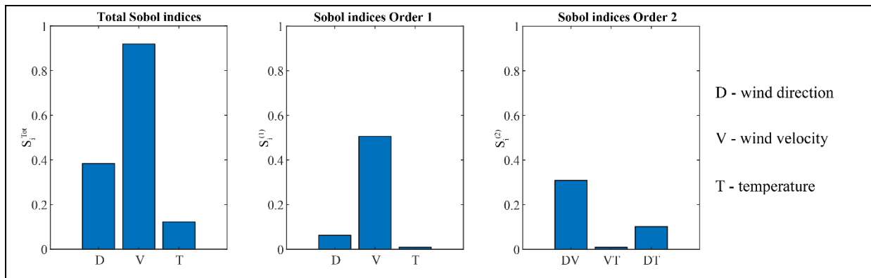
Figure 4.4. Calculated PCE-based Sobol indices
