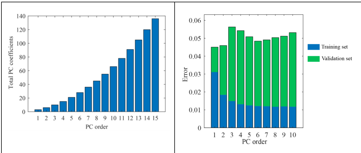
Figure 3.5. (Left) Number of unknown PC coefficients in correlation to selected maximal PC order; (Right) LOO error in correlation to PC model order for the dam case study
