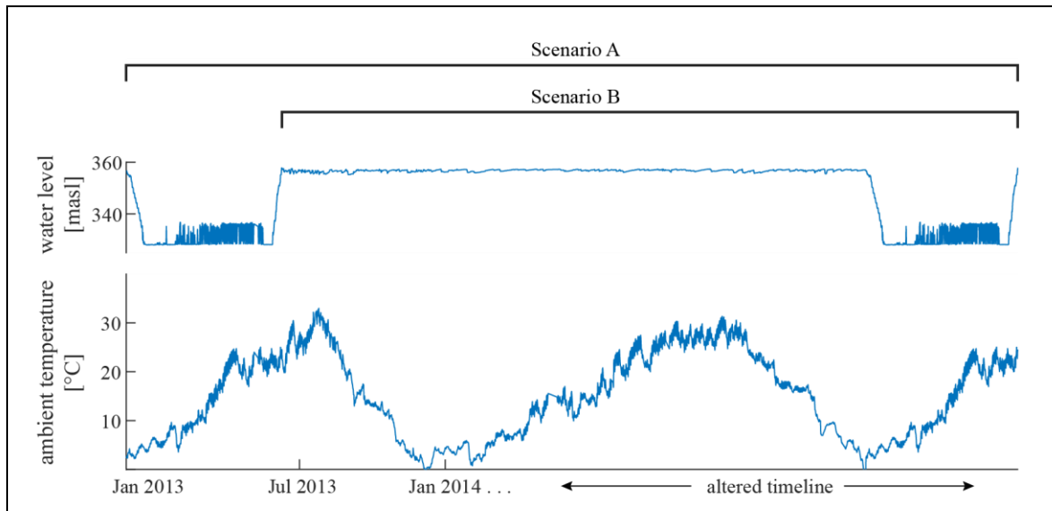
Figure 3.7. Output variables included for training for Scenario A and Scenario B
