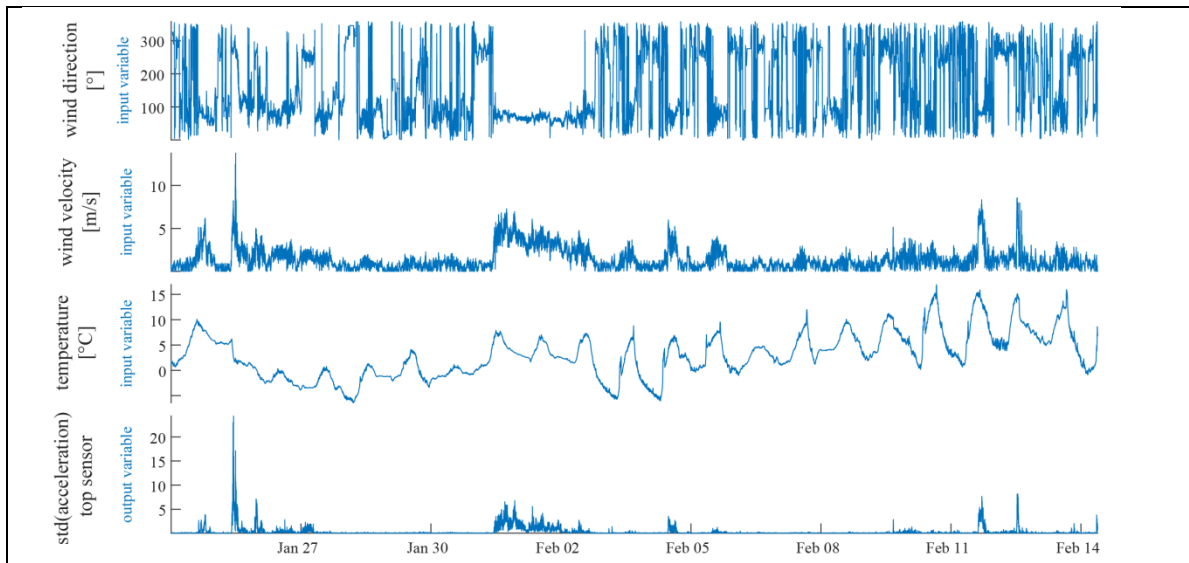
Figure 4.2. Time history plots for measured PCE input and output quantities
