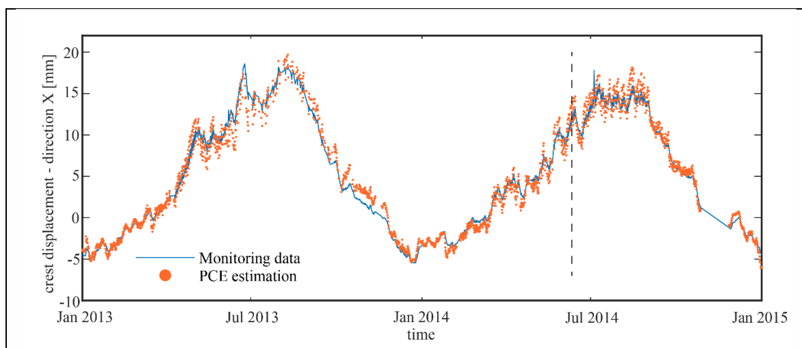
Figure 3.6. Display of output variable and the capability of the PCE model to predict it
