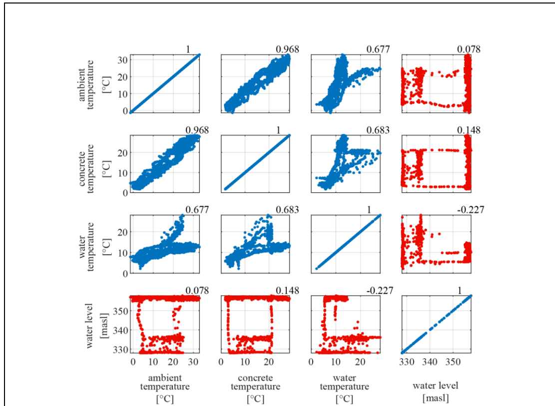
Figure 3.3. Correlation plots for PCE input variables
