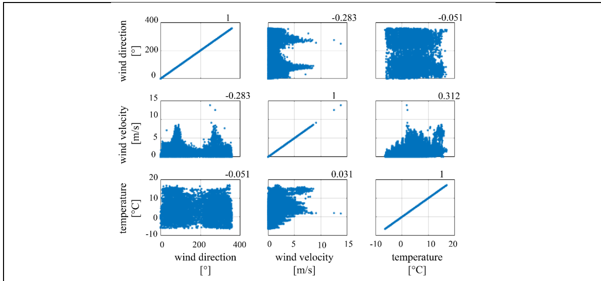
Figure 4.3. Correlation plots for PCE input variables
