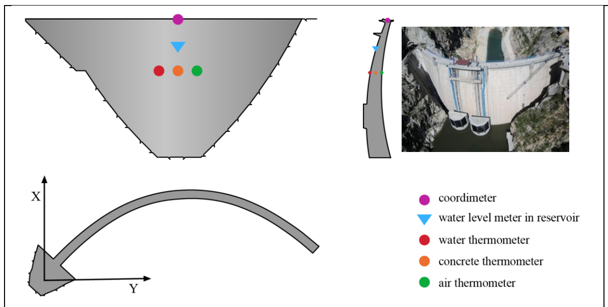
Figure 3.1. The concrete arch dam and a schematic overview of employed sensors from the installed monitoring system
